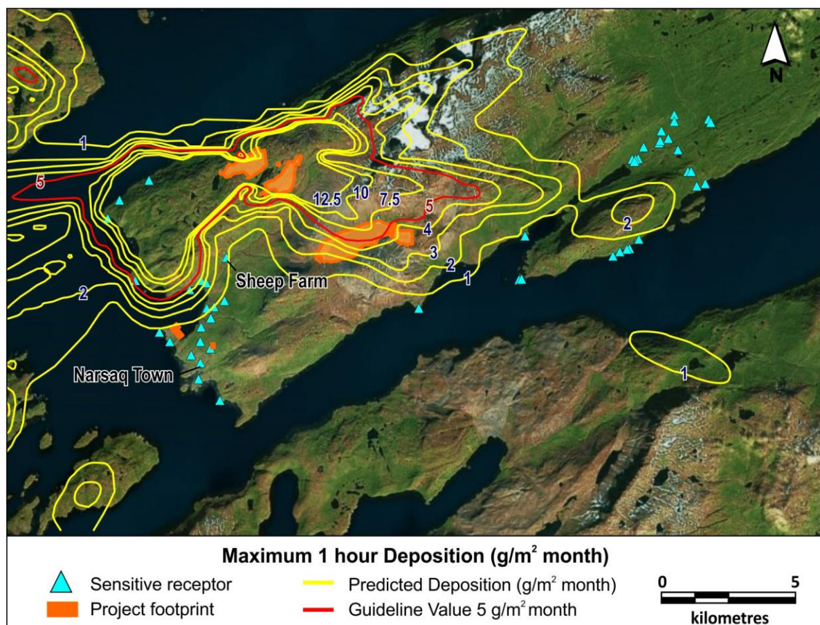
Figure 37 Maximum 1-hour deposition of dust - cumulative (g/m 2 /month)
