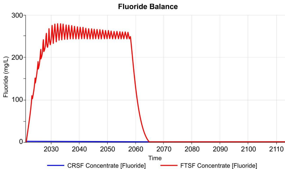
Figure 46 Fluoride (F) Concentrations in both Tailings Facilities of the life of the project as predicted by Goldsim
