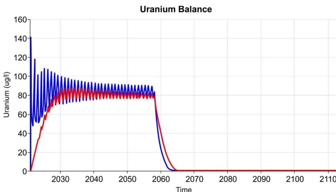
Figure 45 Uranium (U) Concentration in both Tailings Facilities over the life of the project as predicted by Goldsim.
