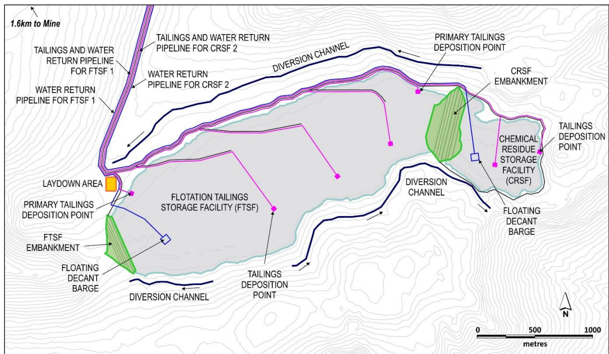
Figure 8 The Tailings Storage Facility
